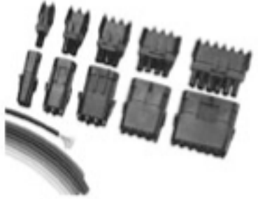
FEMALE PINS MALE PINS CABLE SEAL FEMALE CONNECTOR 1 PIN MALE CONNECTOR 1 PIN FEMALE CONNECTOR 2 PIN MALE CONNECTOR 2 PIN FEMALE CONNECTOR 3 PIN MALE CONNECTOR 3 PIN FEMALE CONNECTOR 4 PIN MALE CONNECTOR 4 PIN FEMALE CONNECTOR 6 PIN MALE CONNECTOR 6 PIN
