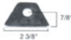
SEAT TAB 1/8" STEEL 1/2" HOLE 3/16" STEEL 1/2" HOLE 1/4" STEEL 1/2" HOLE 1/4" ALUMINUM 1/2" HOLE
