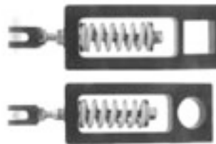
AFCO ALUMINUM 6TH COIL ASSEMBLY 1-1/2 MOUNT 400 LB SPRING ROUND MT. 600 LB SPRING ROUND MT. 400 LB SPRING SQUARE MT. 600 LB SPRING SQUARE MT.
